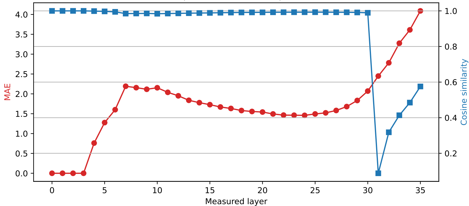
Qwen2.5-3B | Quantized layer 3 | float16 \rightarrow int4
