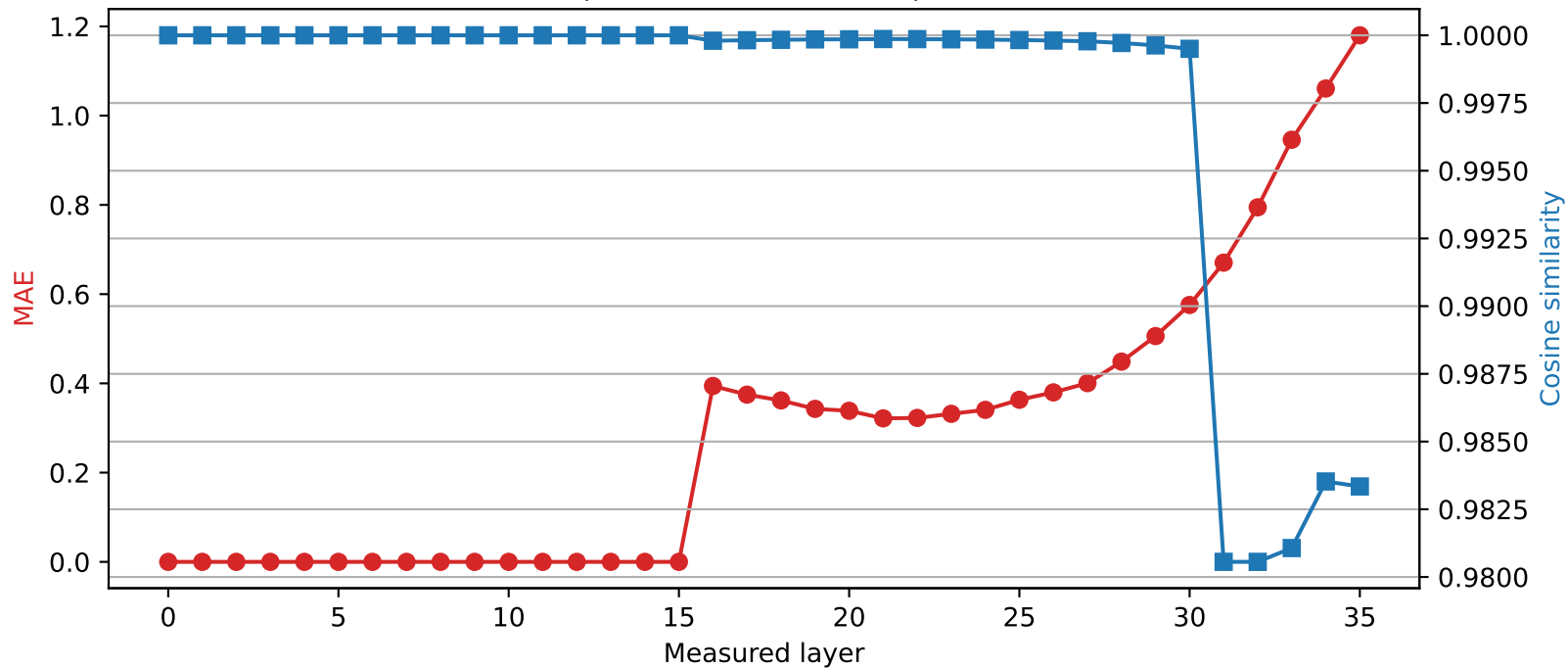
Qwen2.5-3B | Quantized layer 15 | float16 → int4
