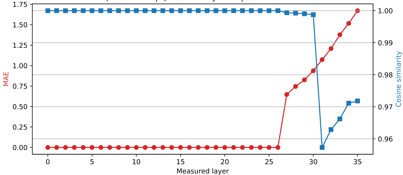
Qwen2.5-3B | Quantized layer 26 | float16 \rightarrow int4
