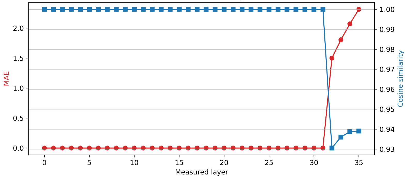
Qwen2.5-3B | Quantized layer 31 | float16 \rightarrow int4
