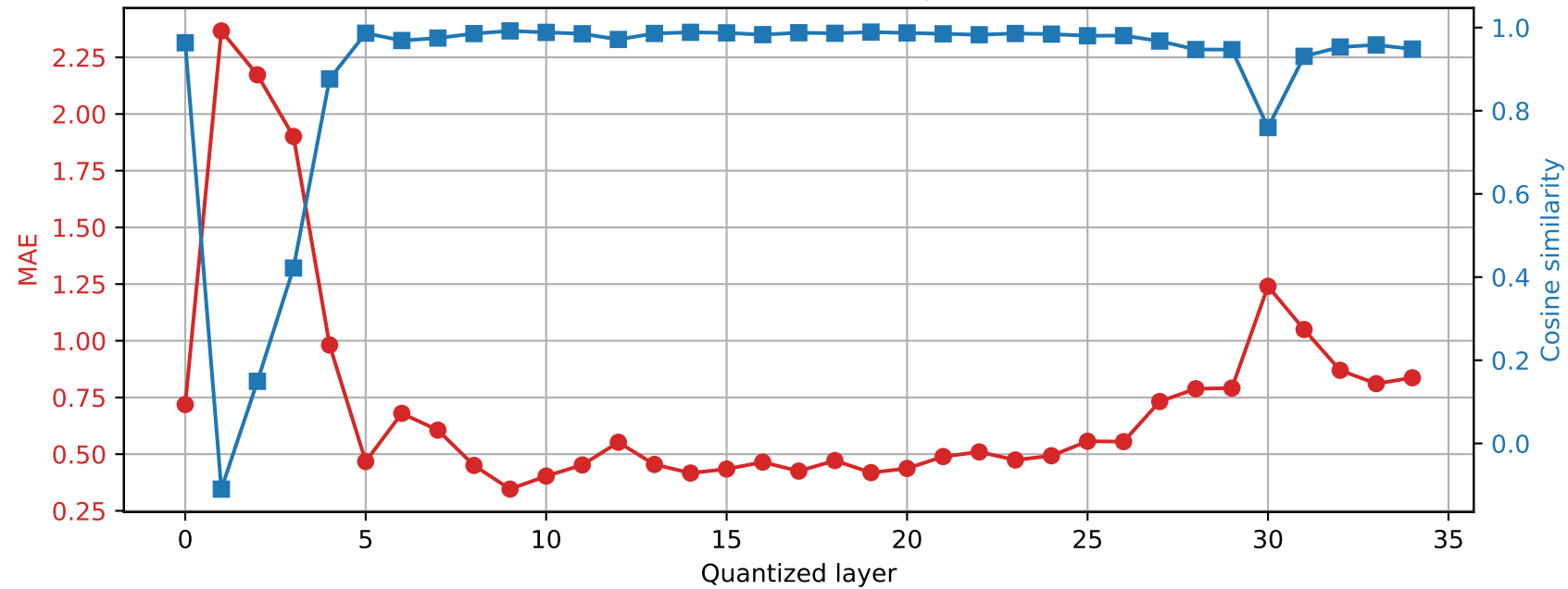
Qwen2.5-3B | Prompt 2 Final RMSNorm output damage | float16 \rightarrow int4
