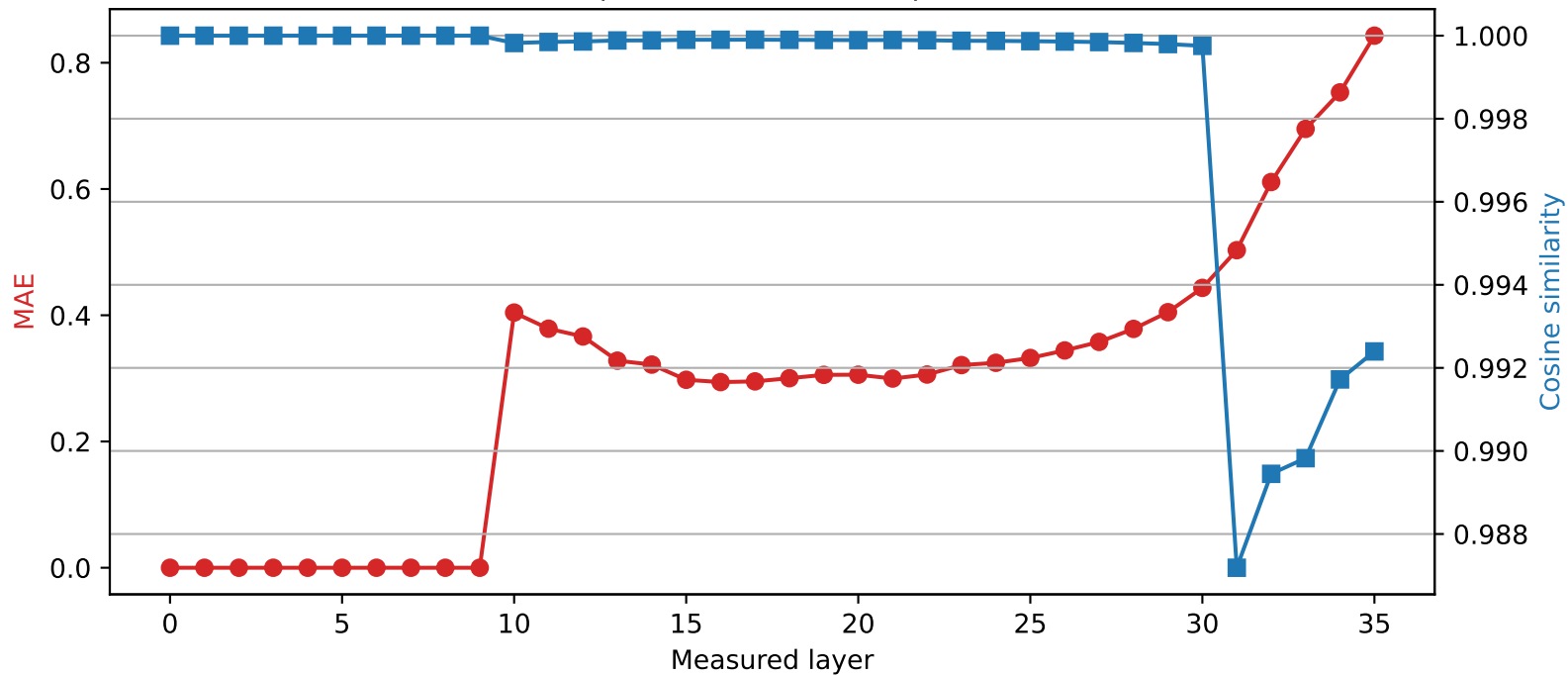
Qwen2.5-3B | Quantized layer 9 | float16 → int4
