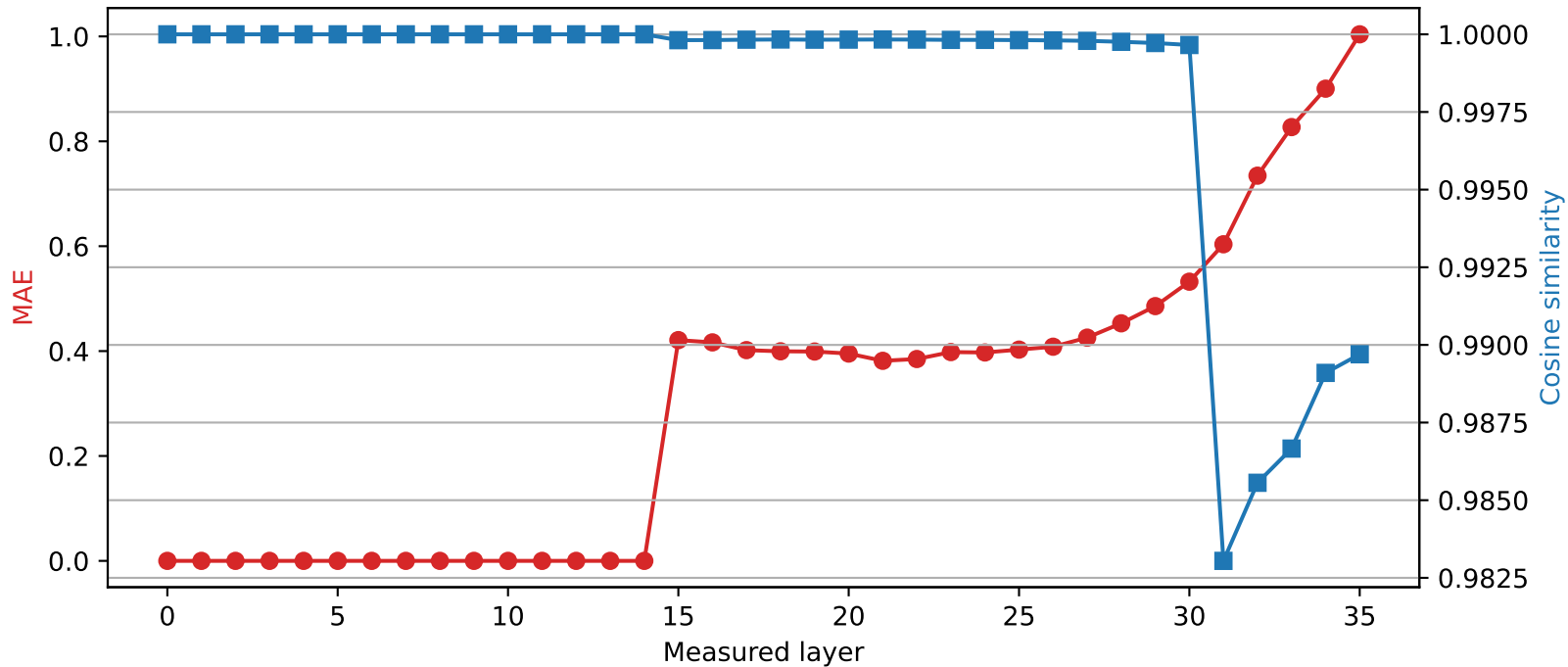
Qwen2.5-3B | Quantized layer 14 | float16 \rightarrow int4
