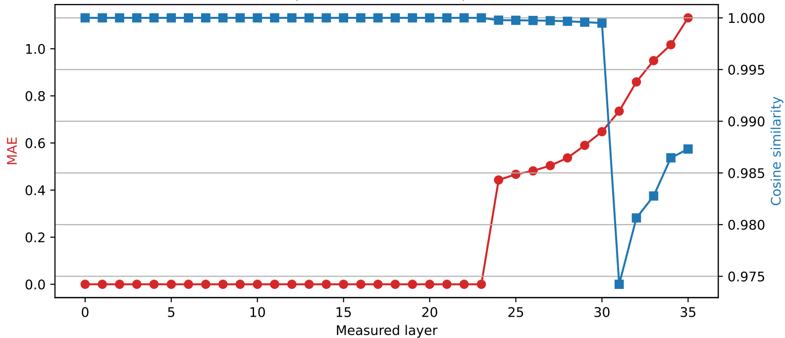
Qwen2.5-3B | Quantized layer 23 | float16 → int4
