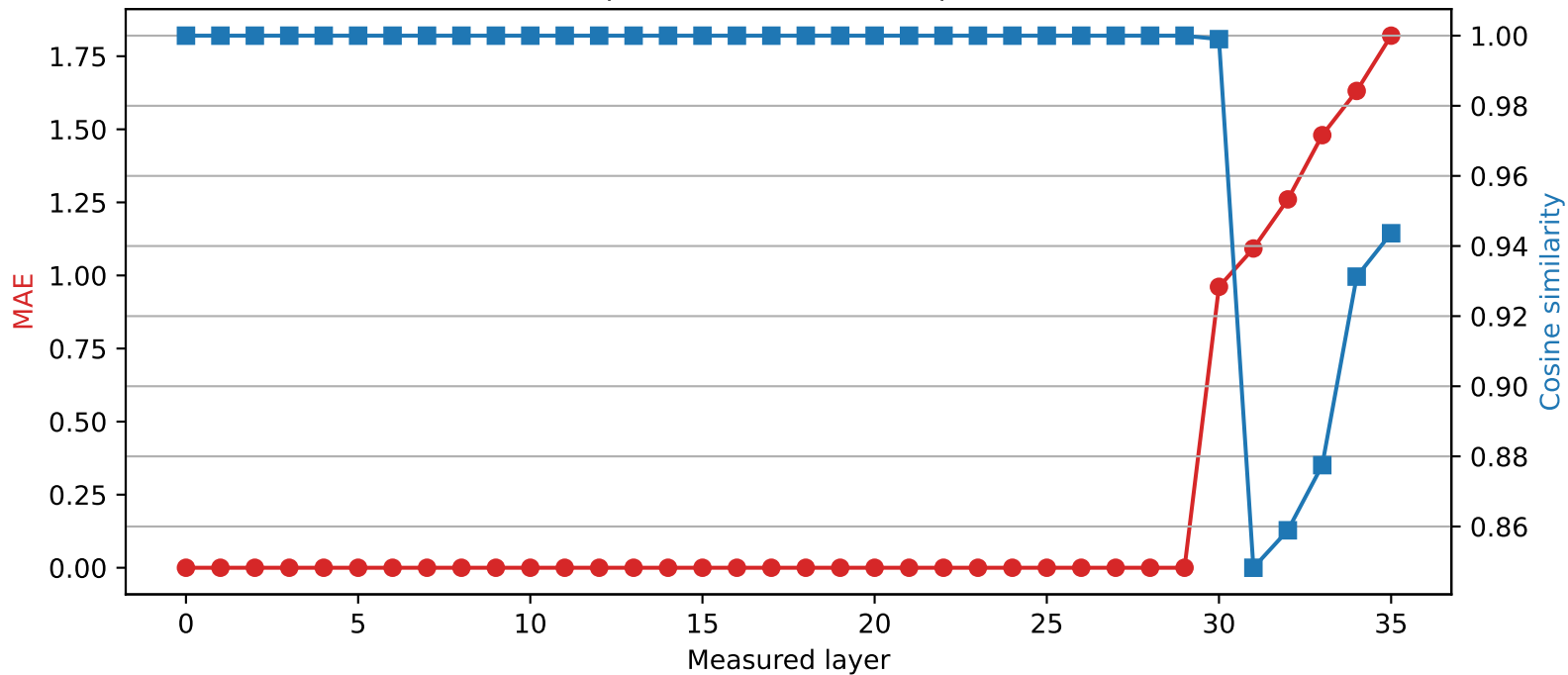
Qwen2.5-3B | Quantized layer 29 | float16 \rightarrow int4
