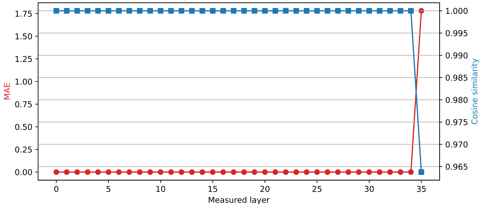
Qwen2.5-3B | Quantized layer 34 | float16 → int4
