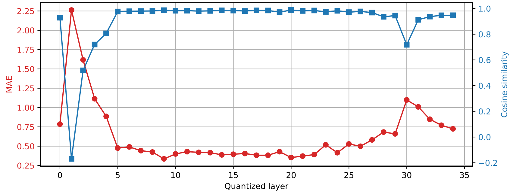
Qwen2.5-3B | Prompt 3 Final RMSNorm output damage | float16 \rightarrow int4
