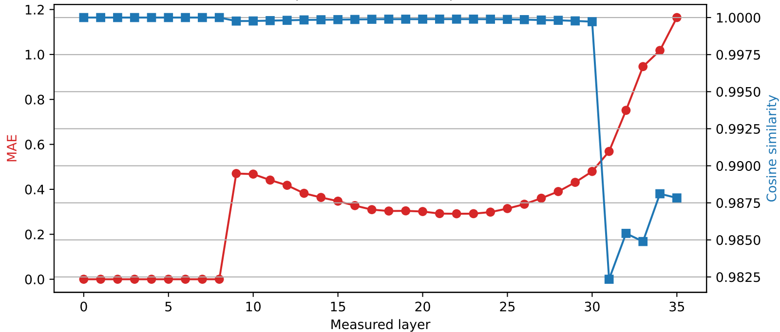
Qwen2.5-3B | Quantized layer 8 | float16 \rightarrow int4
