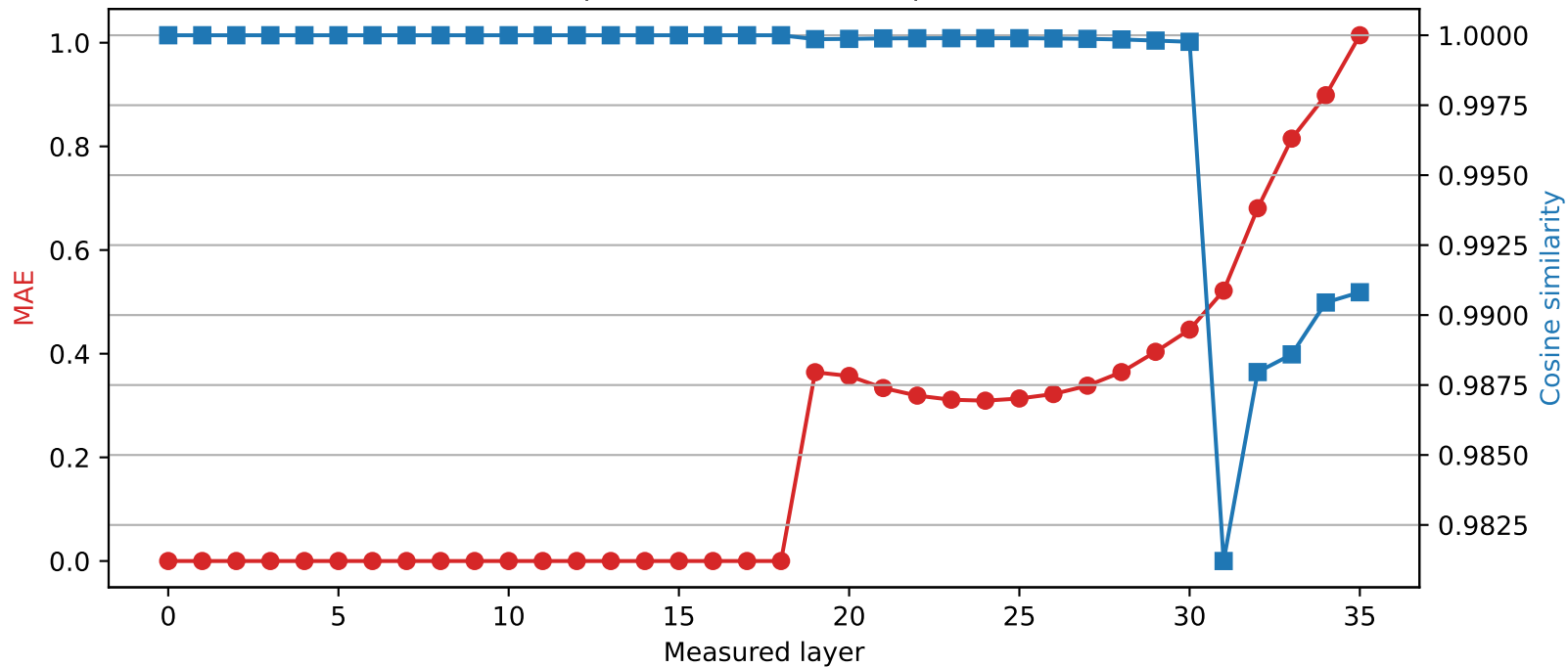
Qwen2.5-3B | Quantized layer 18 | float16 → int4
