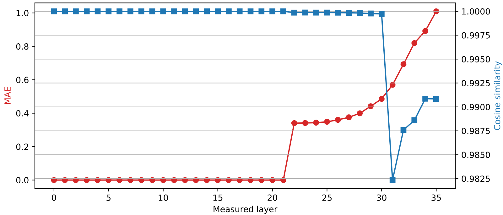
Qwen2.5-3B | Quantized layer 21 | float16 → int4
