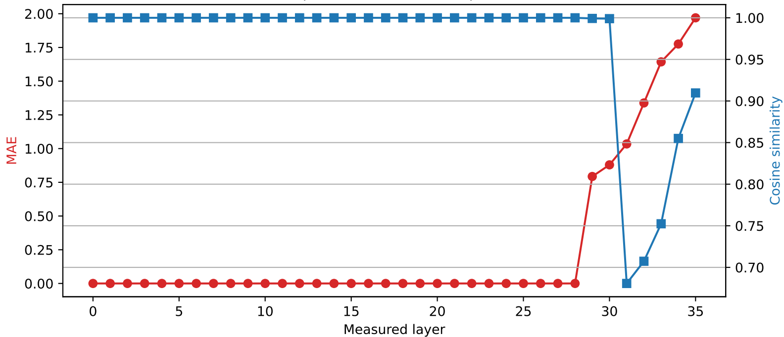
Qwen2.5-3B | Quantized layer 28 | float16 → int4
