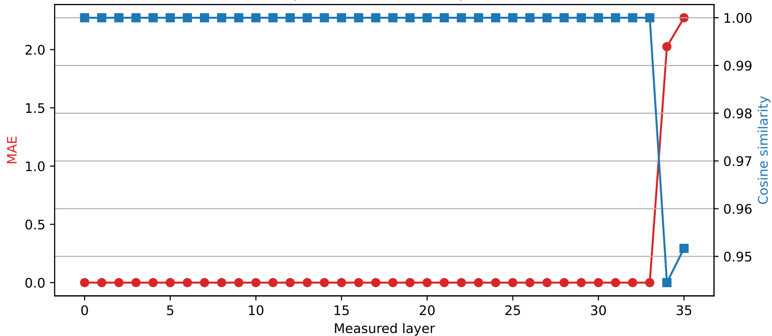
Qwen2.5-3B | Quantized layer 33 | float16 \rightarrow int4
