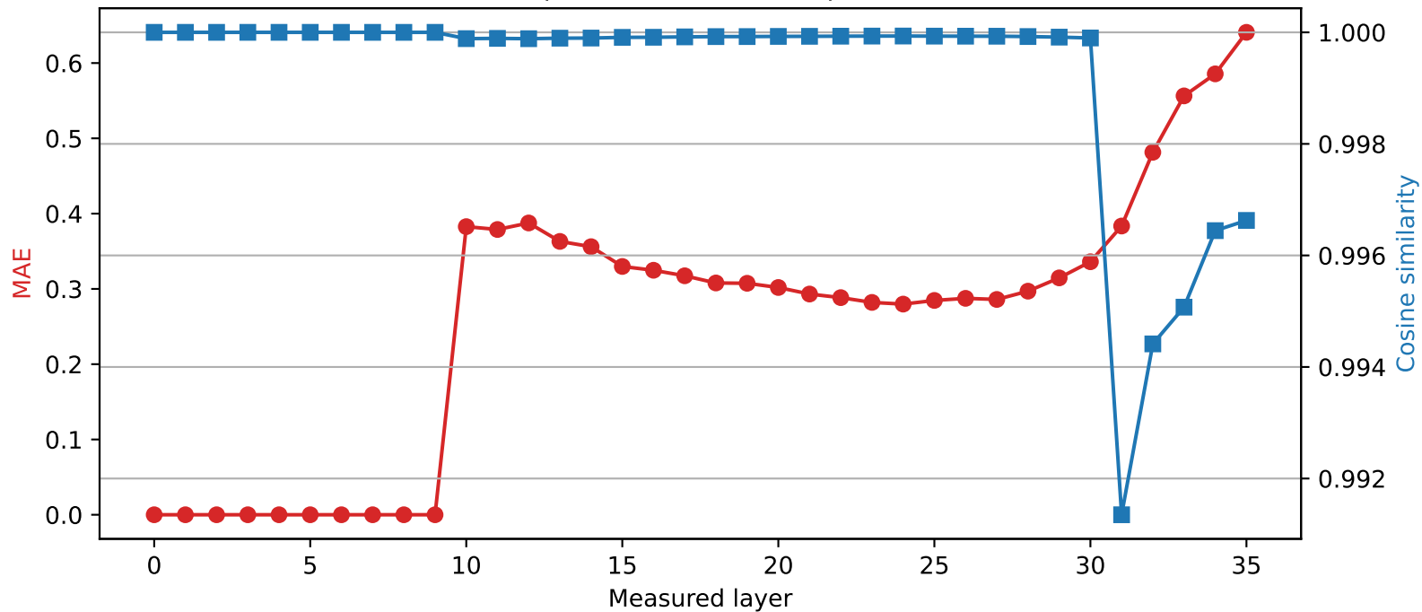
Qwen2.5-3B | Quantized layer 9 | float16 \rightarrow int4
