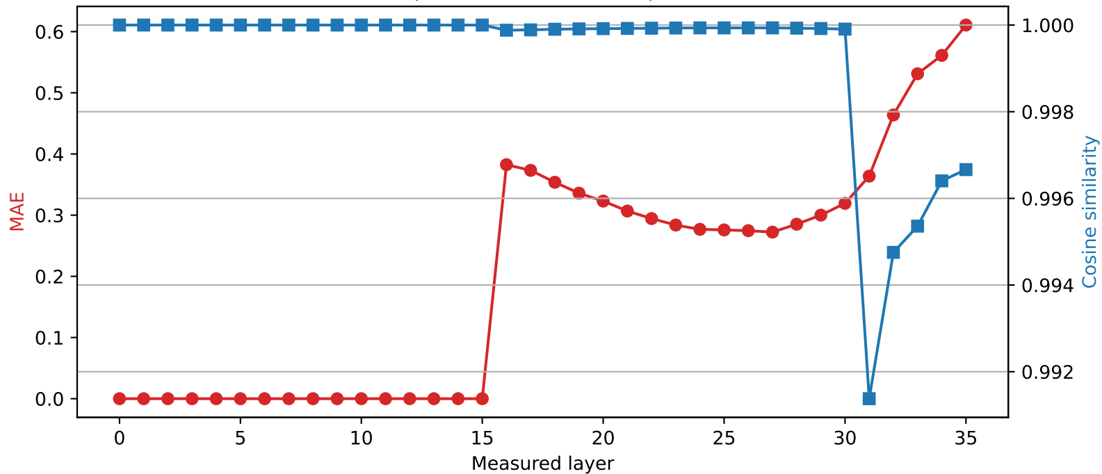
Qwen2.5-3B | Quantized layer 15 | float16 \rightarrow int4
