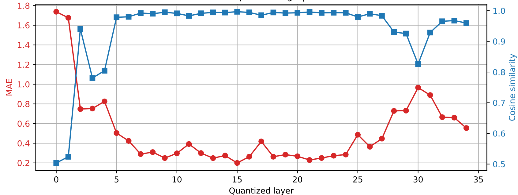
Qwen2.5-3B | Prompt 0 Final RMSNorm output damage | float16 \rightarrow int2
