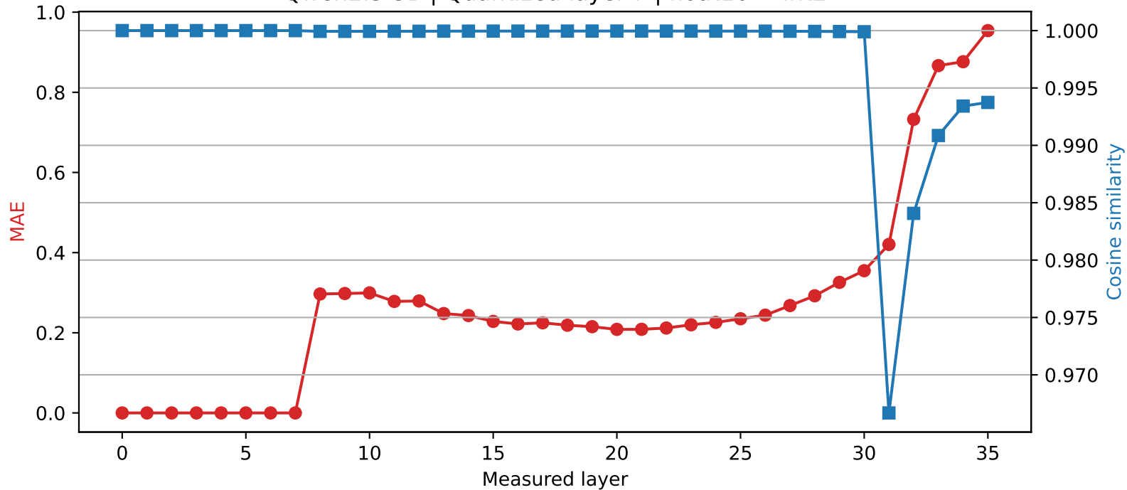
Qwen2.5-3B | Quantized layer 7 | float16 \rightarrow int2
