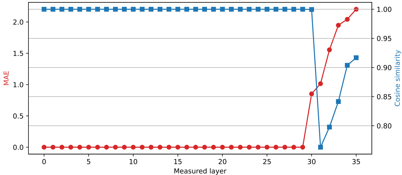
Qwen2.5-3B | Quantized layer 29 | float16 \rightarrow int2
