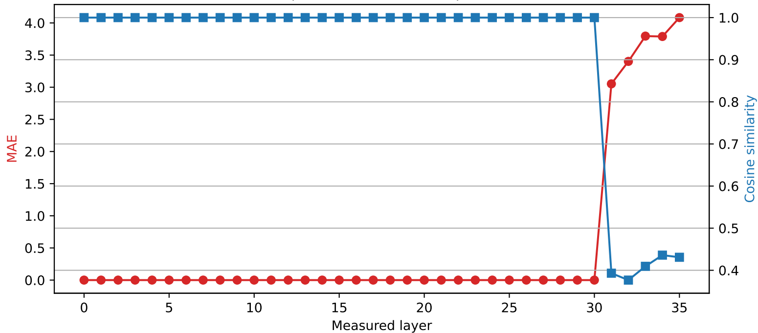
Qwen2.5-3B | Quantized layer 30 | float16 \rightarrow int2
