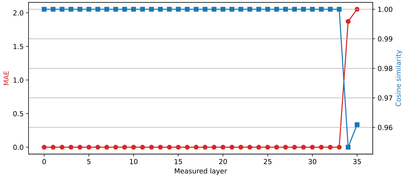
Qwen2.5-3B | Quantized layer 33 | float16 \rightarrow int2
