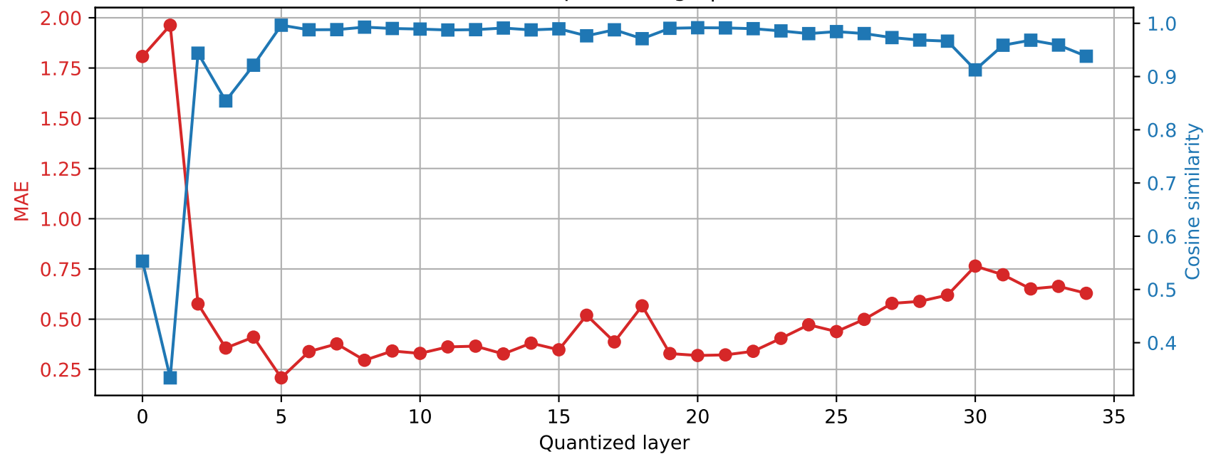
Qwen2.5-3B | Prompt 1 Final RMSNorm output damage | float16 \rightarrow int2
