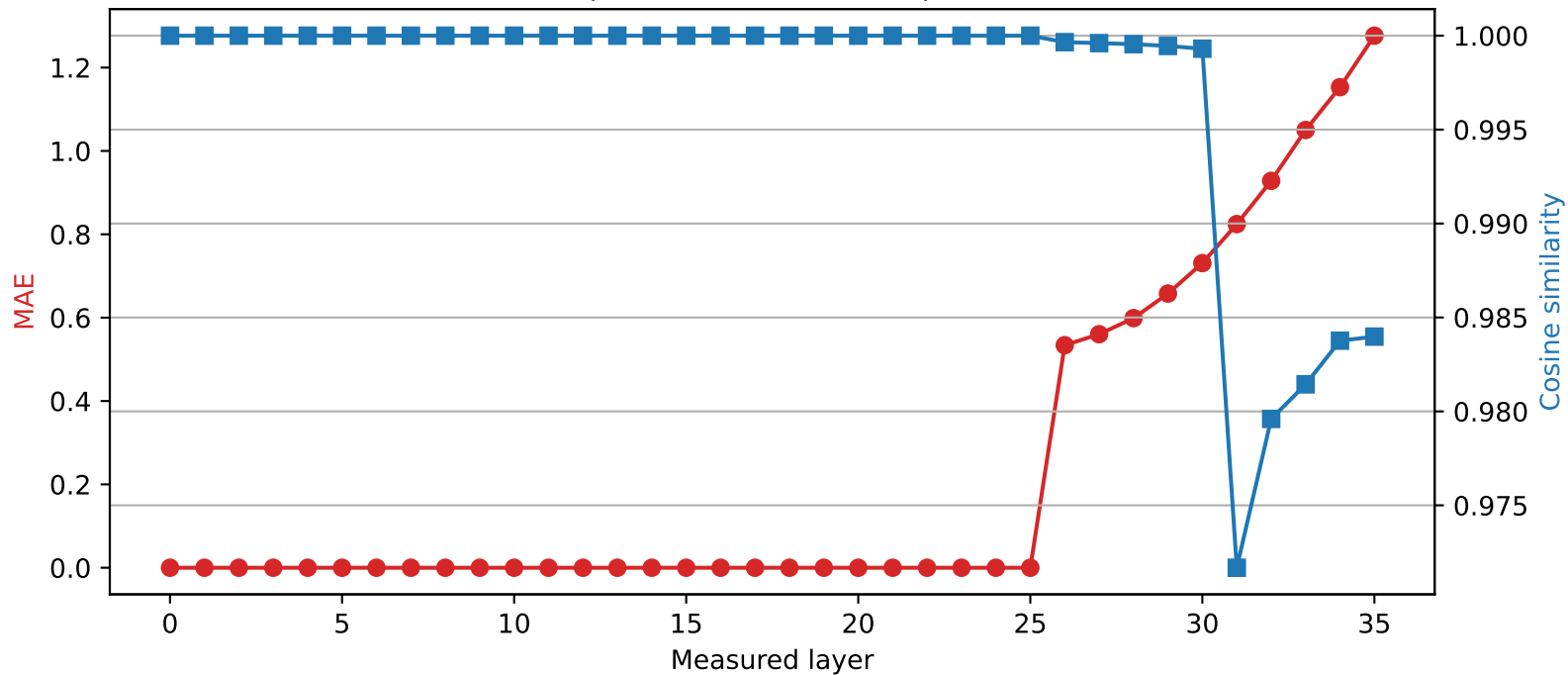
Qwen2.5-3B | Quantized layer 25 | float16 → int2
