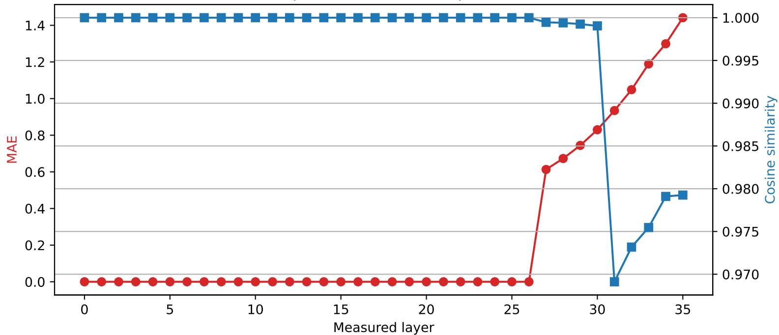
Qwen2.5-3B | Quantized layer 26 | float16 \rightarrow int2
