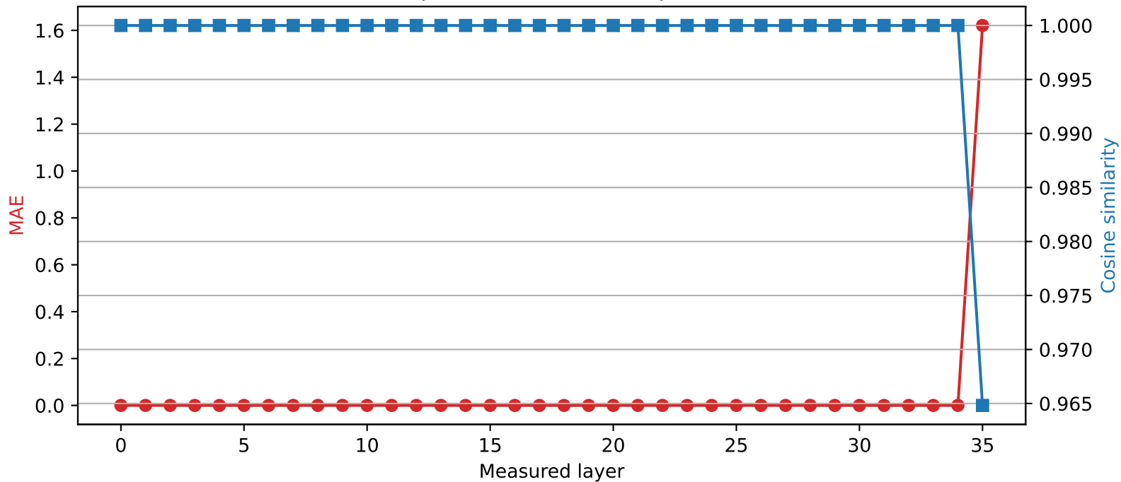
Qwen2.5-3B | Quantized layer 34 | float16 → int2
