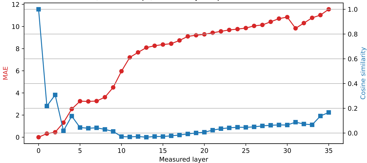
Qwen2.5-3B | Quantized layer 0 | float16 \rightarrow int2
