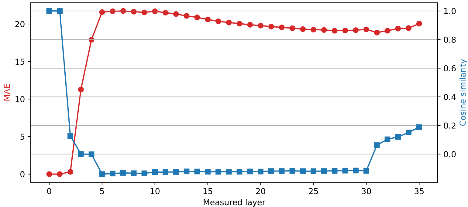
Qwen2.5-3B | Quantized layer 1 | float16 \rightarrow int2
