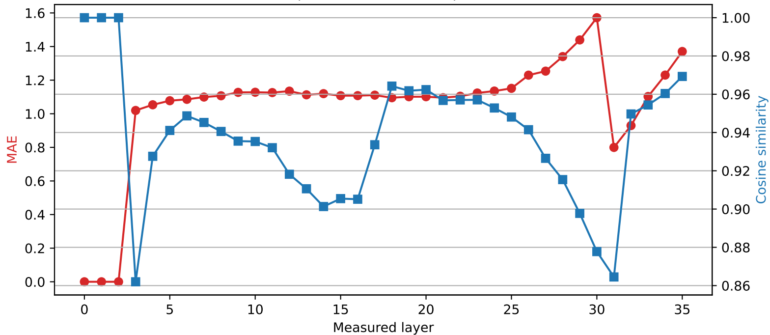
Qwen2.5-3B | Quantized layer 2 | float16 → int2
