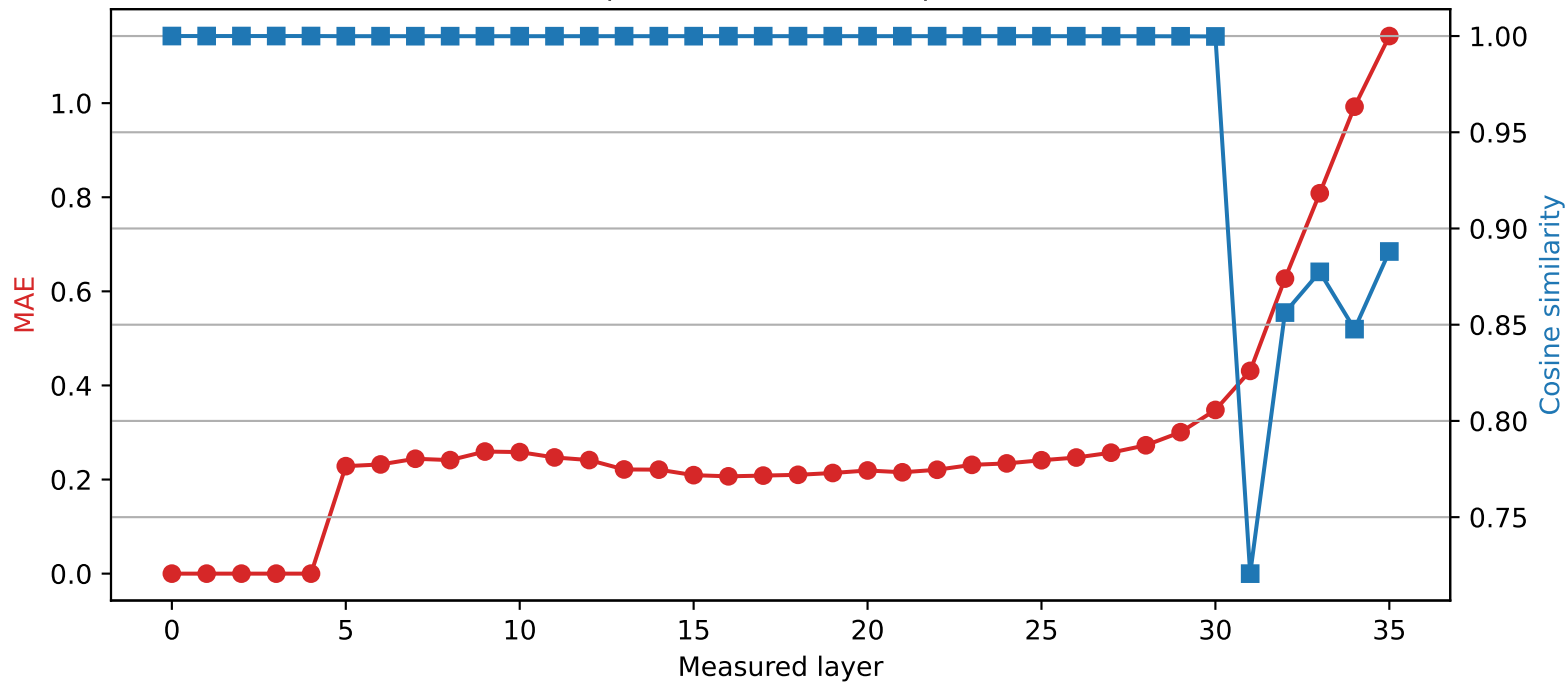
Qwen2.5-3B | Quantized layer 4 | float16 → int2
