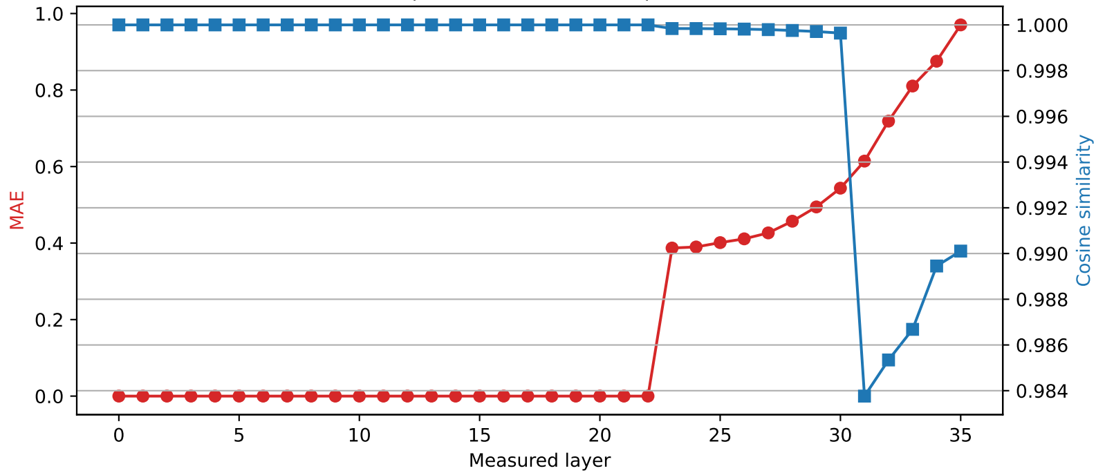
Qwen2.5-3B | Quantized layer 22 | float16 \rightarrow int2
