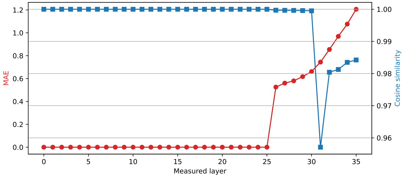
Qwen2.5-3B | Quantized layer 25 | float16 \rightarrow int2
