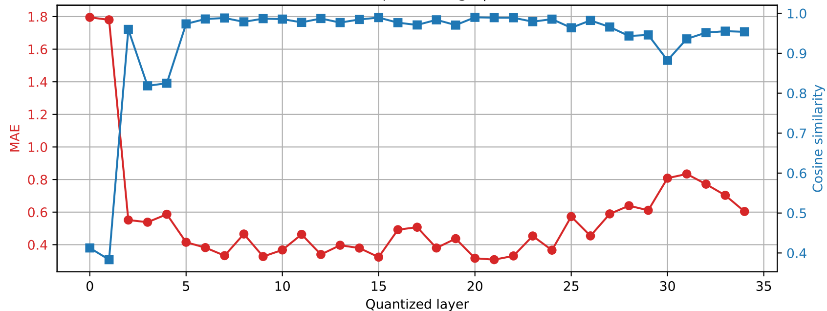
Qwen2.5-3B | Prompt 3 Final RMSNorm output damage | float16 \rightarrow int2
