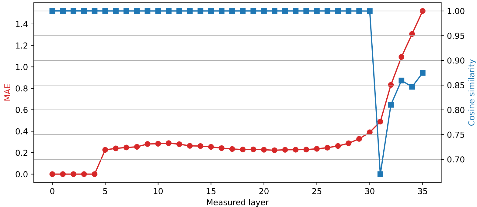
Qwen2.5-3B | Quantized layer 4 | float16 \rightarrow int2
