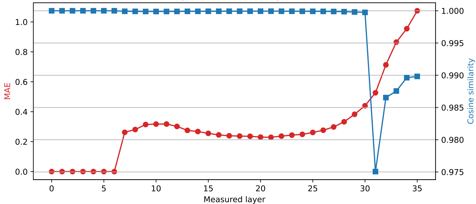
Qwen2.5-3B | Quantized layer 6 | float16 \rightarrow int2
