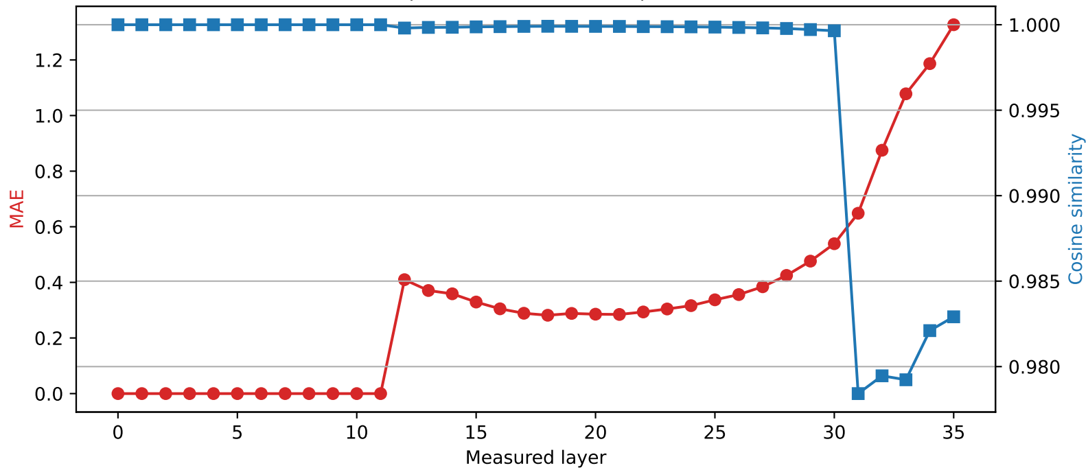
Qwen2.5-3B | Quantized layer 11 | float16 → int2
