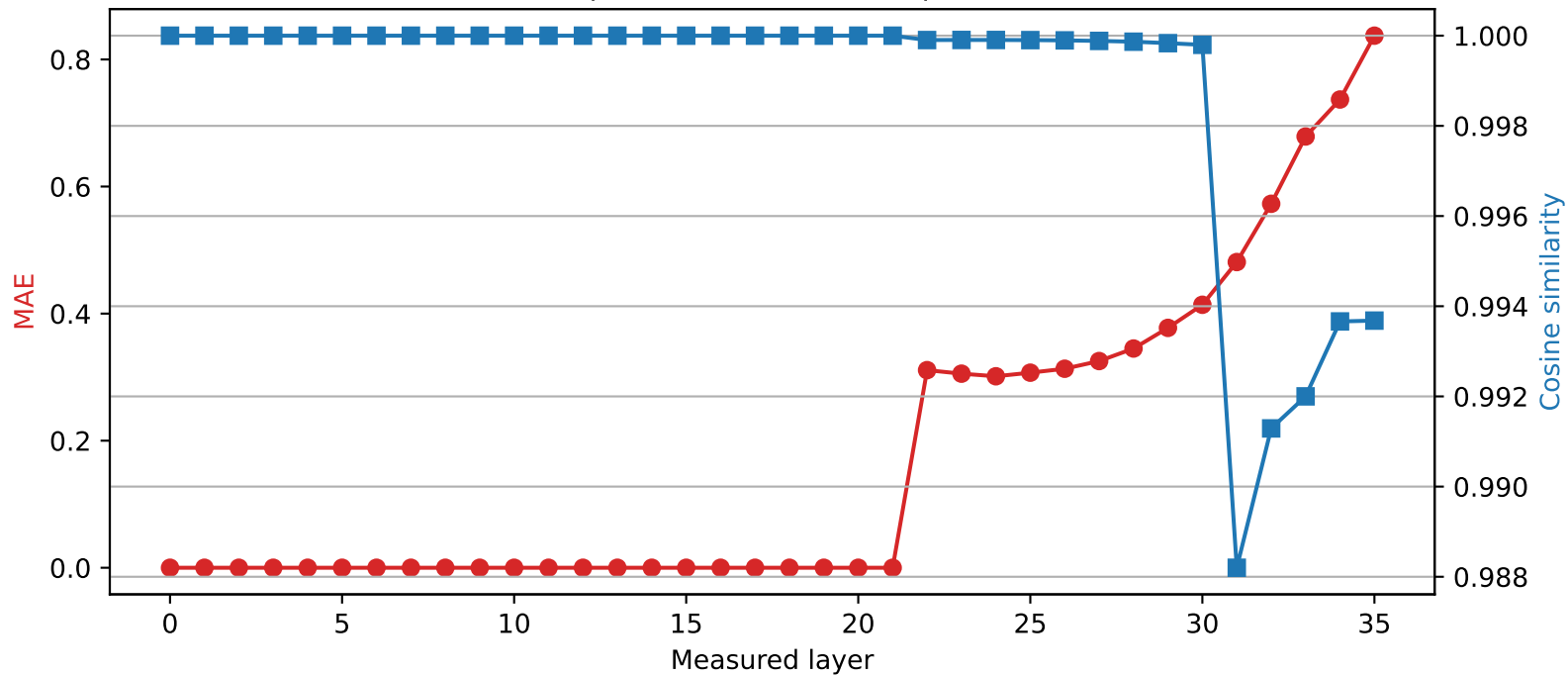
Qwen2.5-3B | Quantized layer 21 | float16 \rightarrow int2
