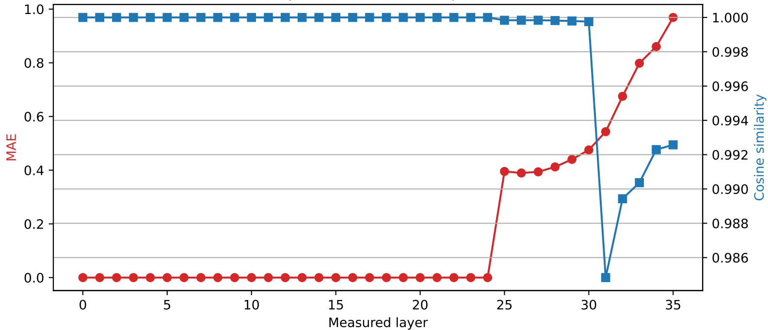
Qwen2.5-3B | Quantized layer 24 | float16 \rightarrow int2
