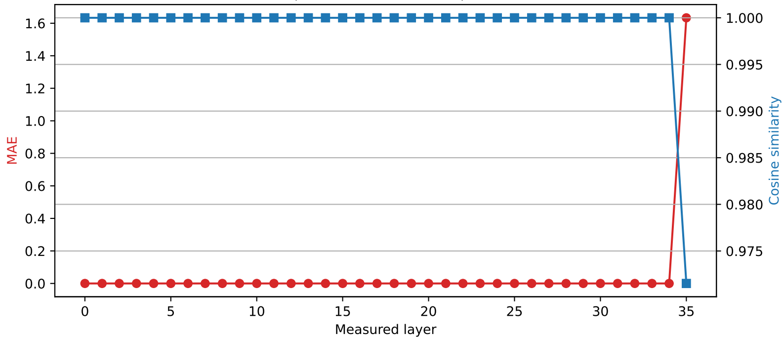
Qwen2.5-3B | Quantized layer 34 | float16 \rightarrow int2
