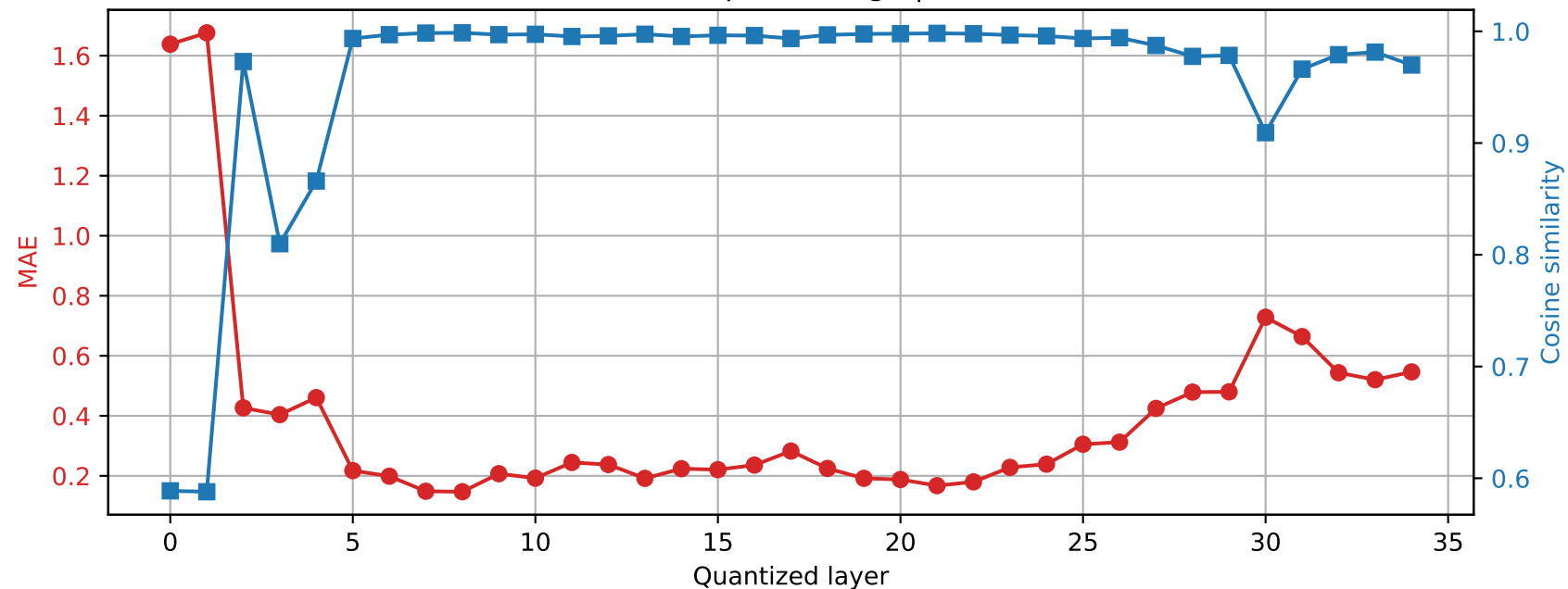
Qwen2.5-3B | Prompt 4 Final RMSNorm output damage | float16 \rightarrow int2
