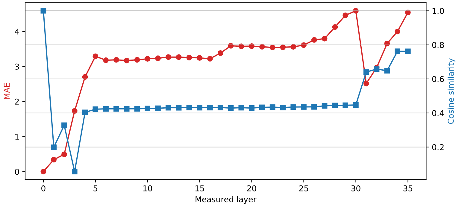
Qwen2.5-3B | Quantized layer 0 | float16 → int2
