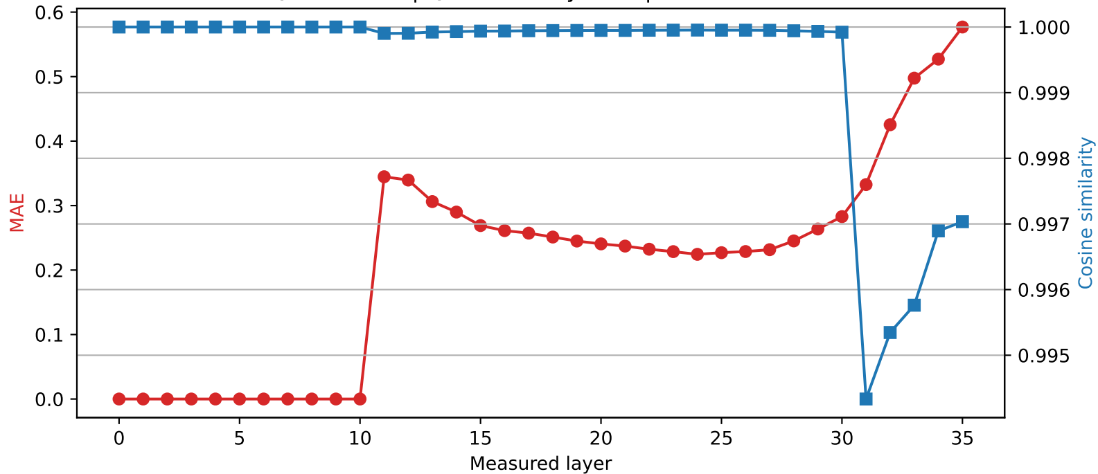
Qwen2.5-3B | Quantized layer 10 | float16 \rightarrow int2
