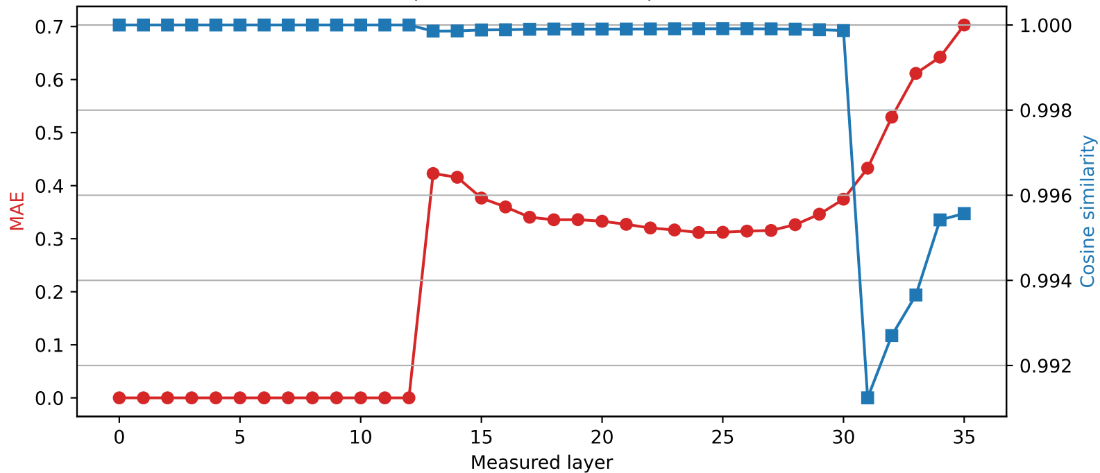
Qwen2.5-3B | Quantized layer 12 | float16 \rightarrow int2
