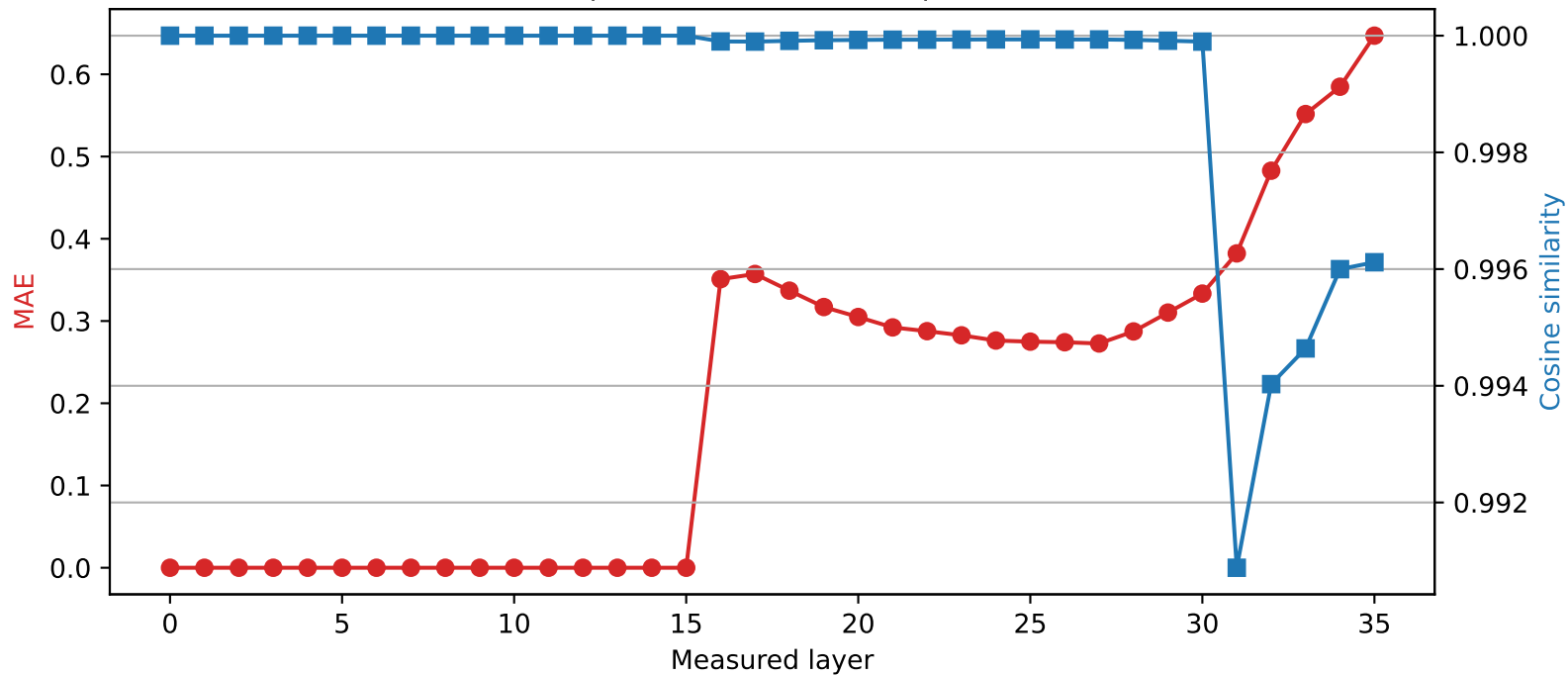
Qwen2.5-3B | Quantized layer 15 | float16 \rightarrow int2
