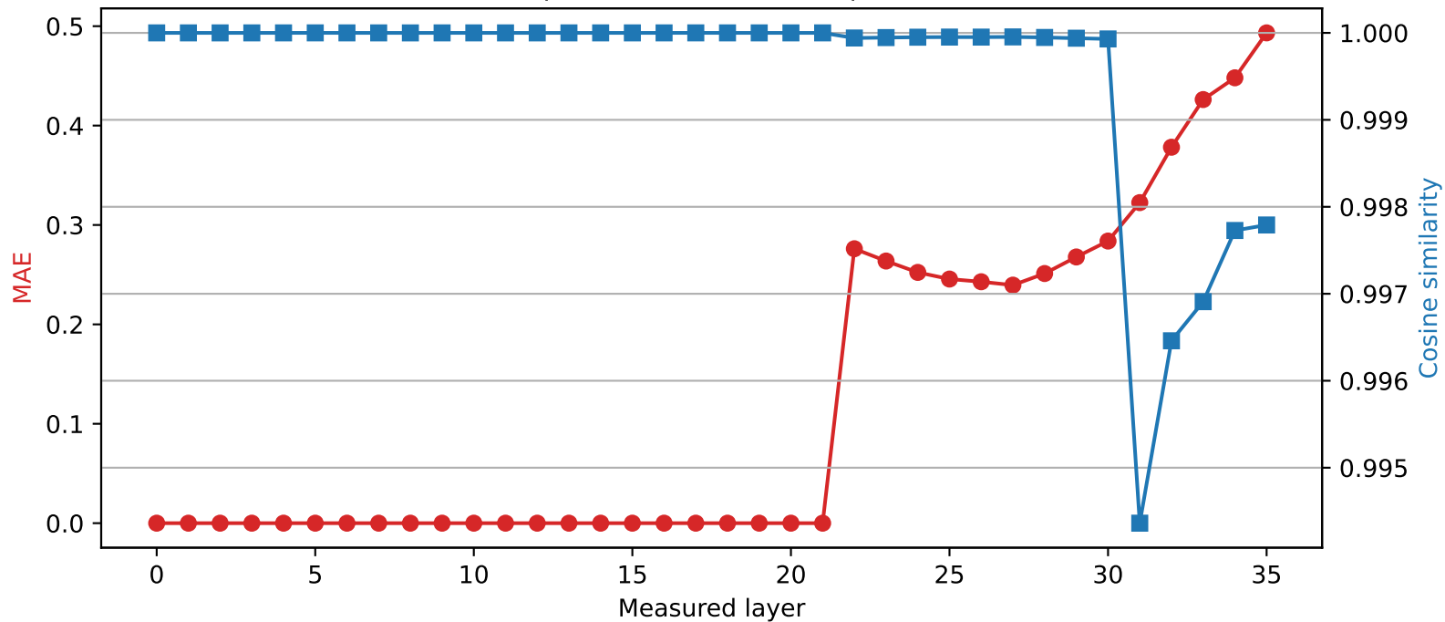
Qwen2.5-3B | Quantized layer 21 | float16 → int2
