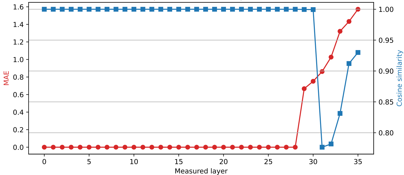
Qwen2.5-3B | Quantized layer 28 | float16 \rightarrow int2
