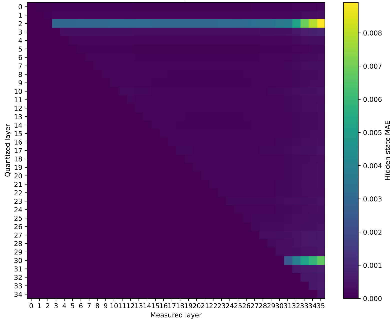
Model: Qwen2.5-3B | float32 → int16
