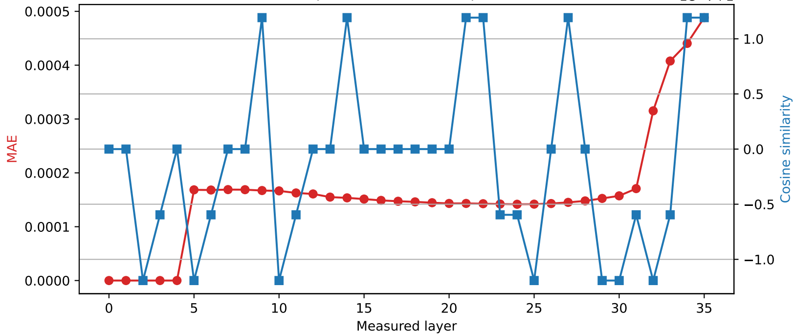
Qwen2.5-3B | Quantized layer 4 | float32 \rightarrow int16
