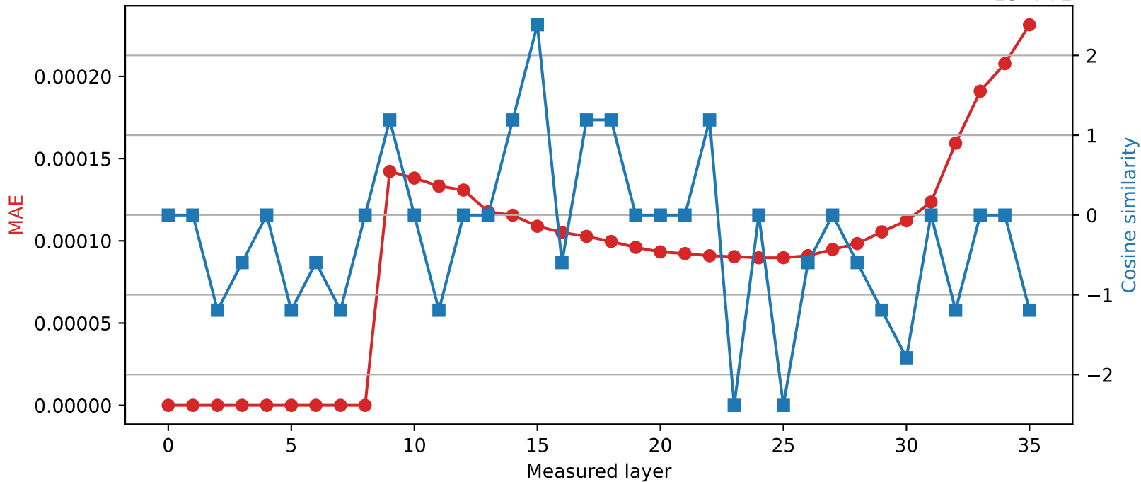
Qwen2.5-3B | Quantized layer 8 | float32 \rightarrow int16
